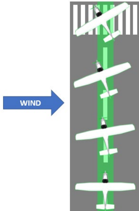
Figure 4.3.2. Crosswind climb flightpath.
